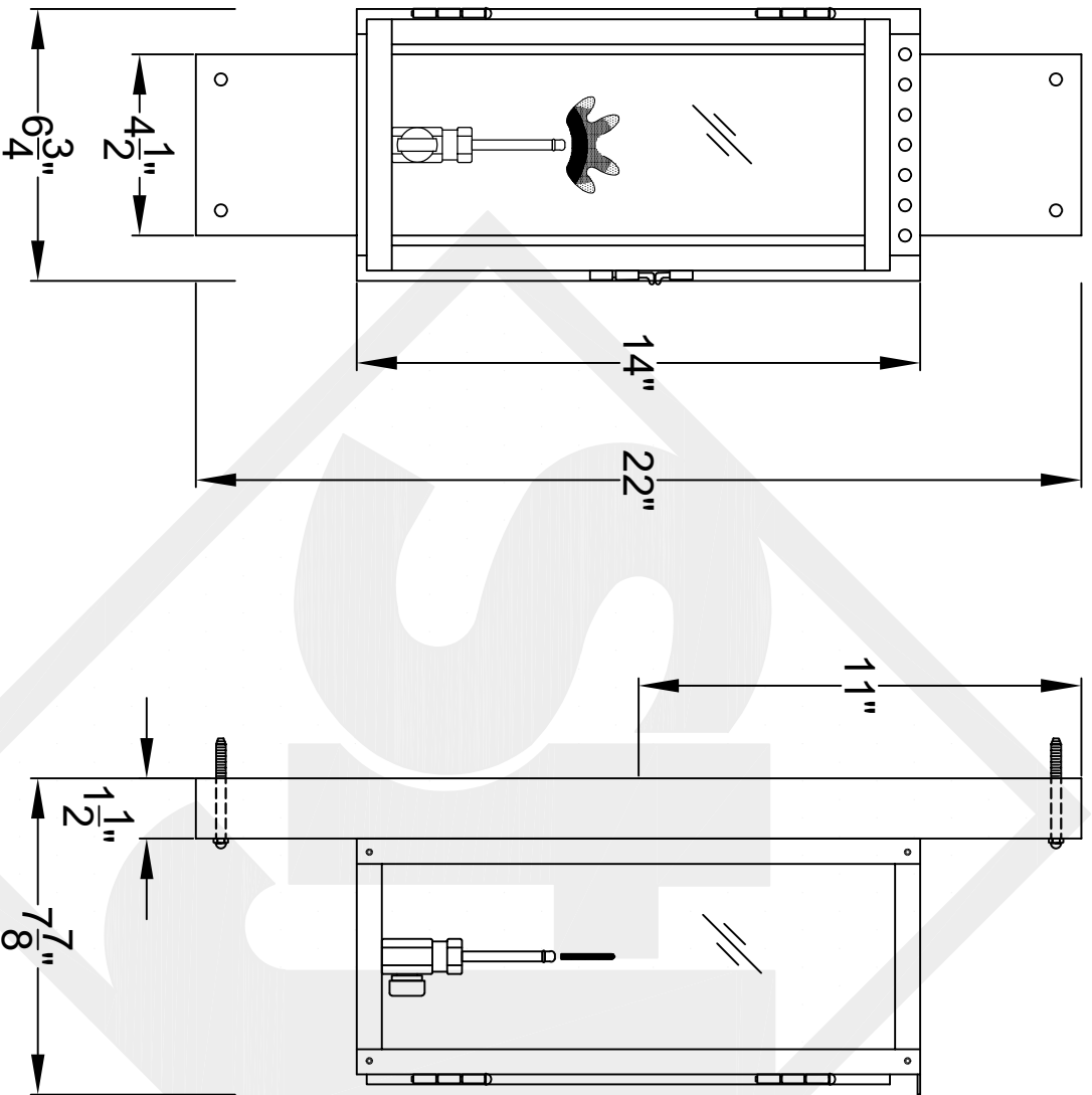
Front View
