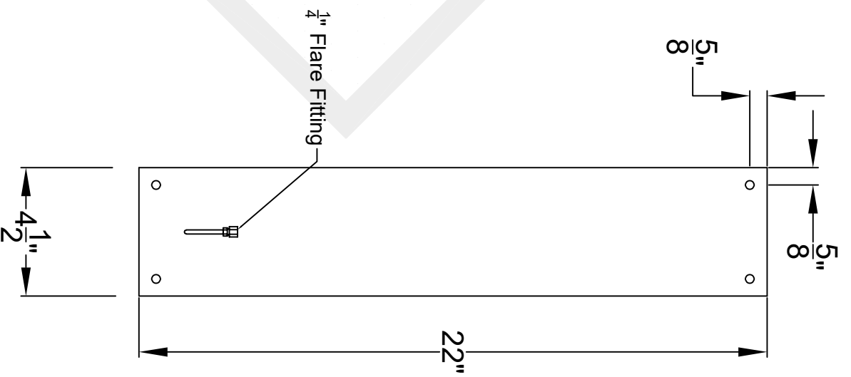
Backplate
