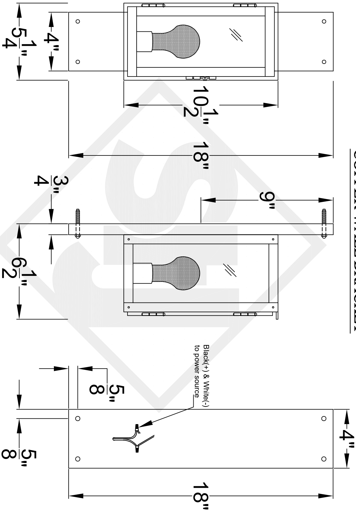
Front View
