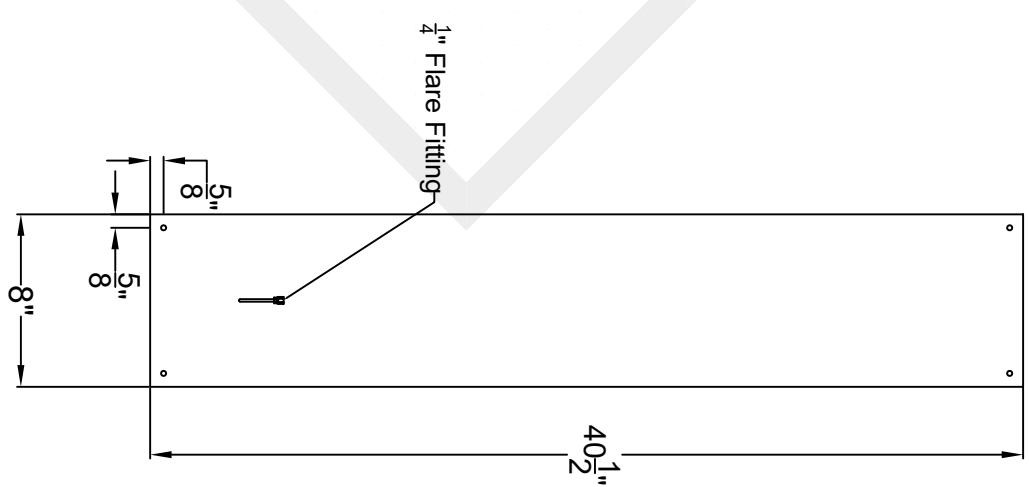
Backplate
